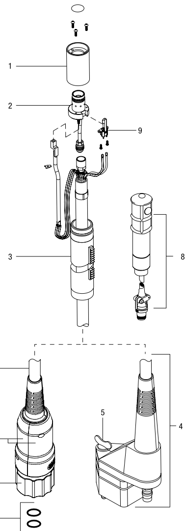
ICE-80CXM Torch
