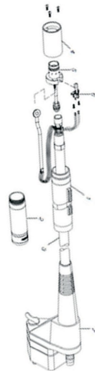
XT60M Torch
