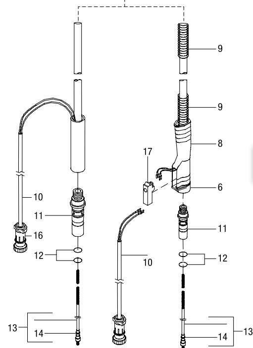
M-10 Gun
