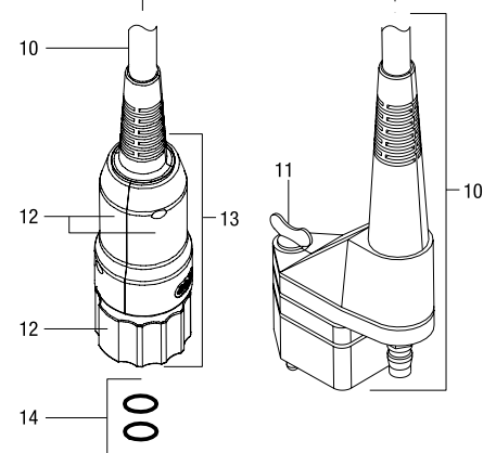
ICE-80CX Torch
