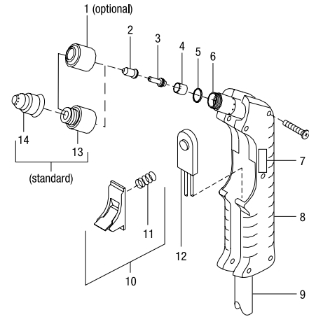
ICE-12C Torch
