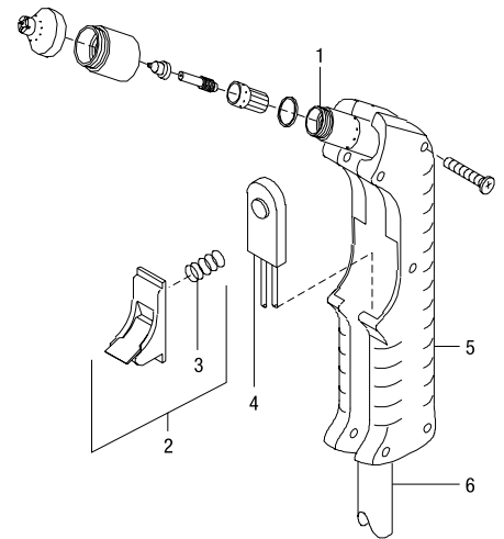
ICE-40C/T Torch
